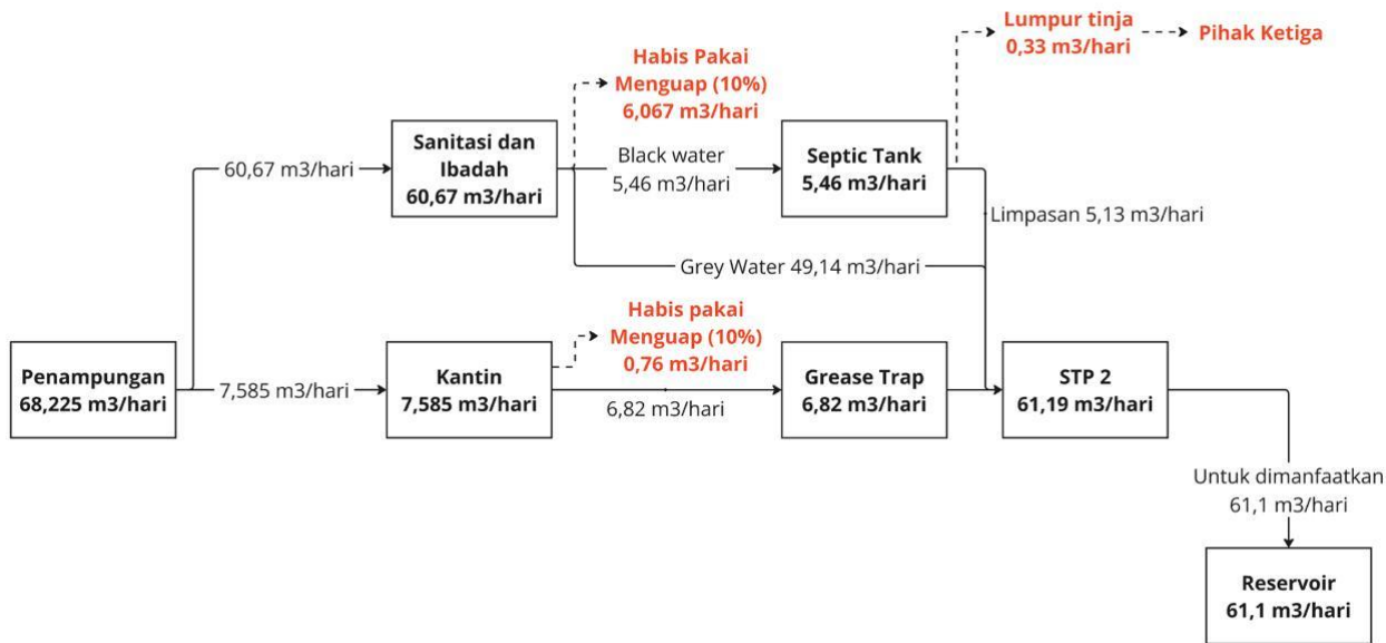
Gambar 3. Neraca Air STP 2
