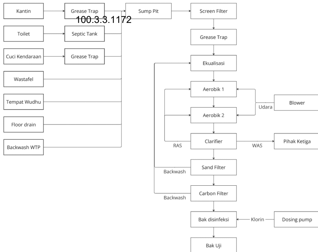
Gambar 5. Diagram Alir STP 1
