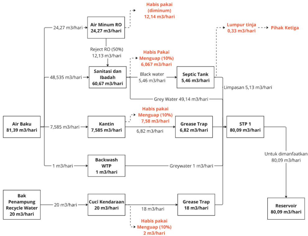
Gambar 2. Neraca Air STP 1
